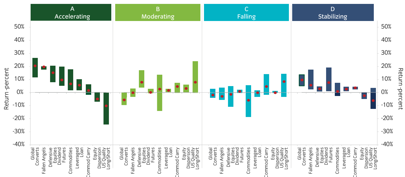
Figure 31: Alternative strategies across growth regimes 33
