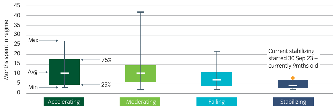
Figure 8: The most persistent regimes have been those where PMIs are above 50 9
