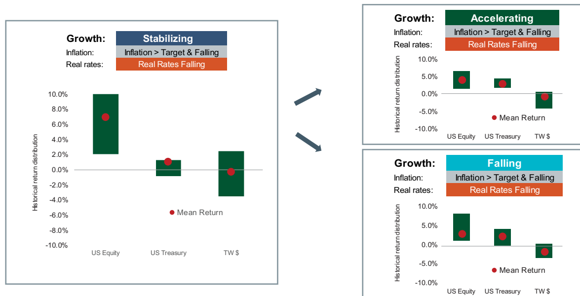
Figure 28: A shift to AFJ would still be positive for equities 30
